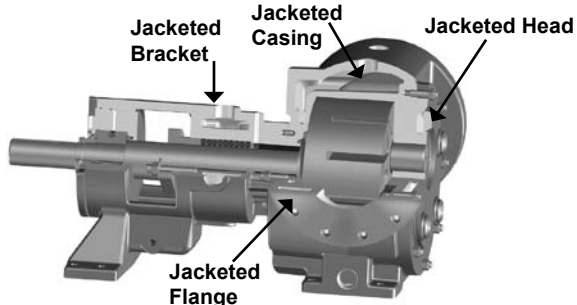
Fully-Jacketed Pump Cutaway – N324A
